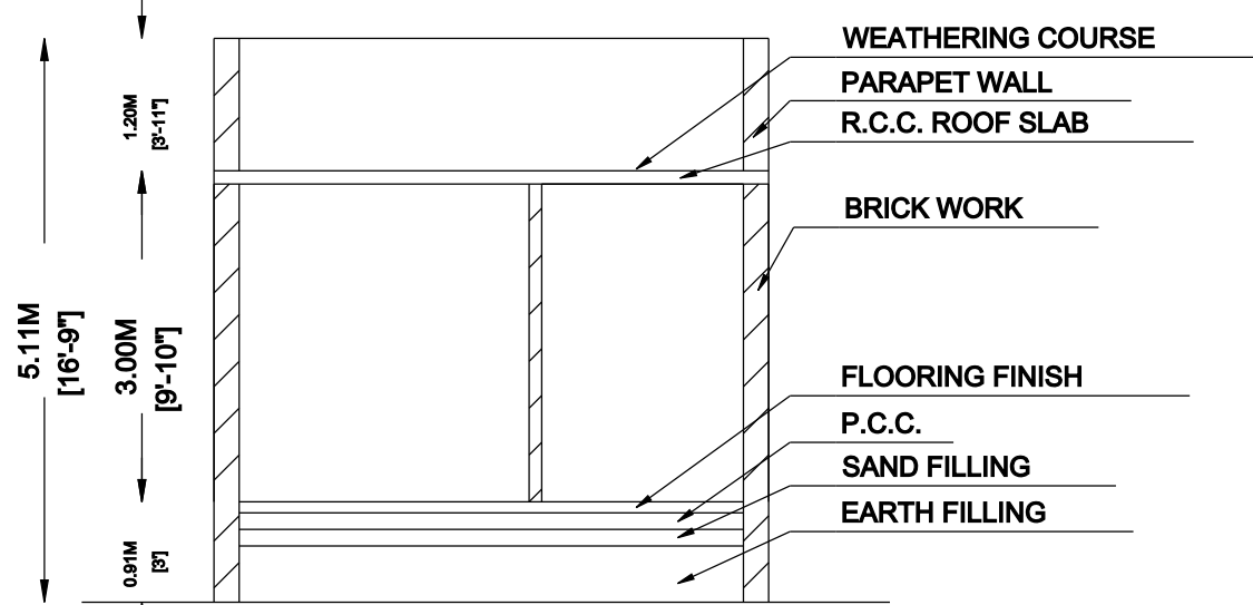
SECTION ON XX
