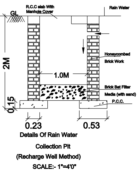
SCALE:- 1"=4V'
