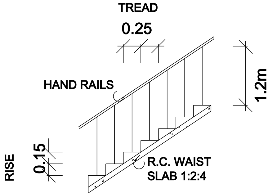
STAIRCASE DETAILS
