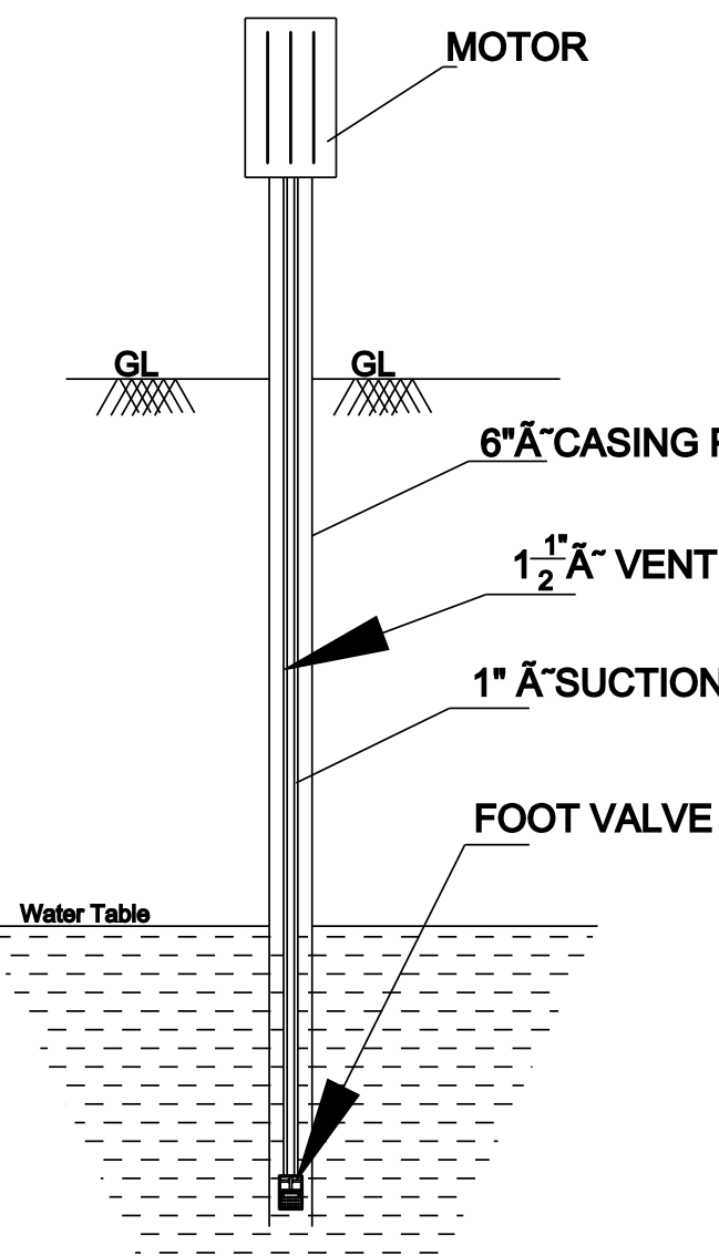
SEC. OF BOREWELL
