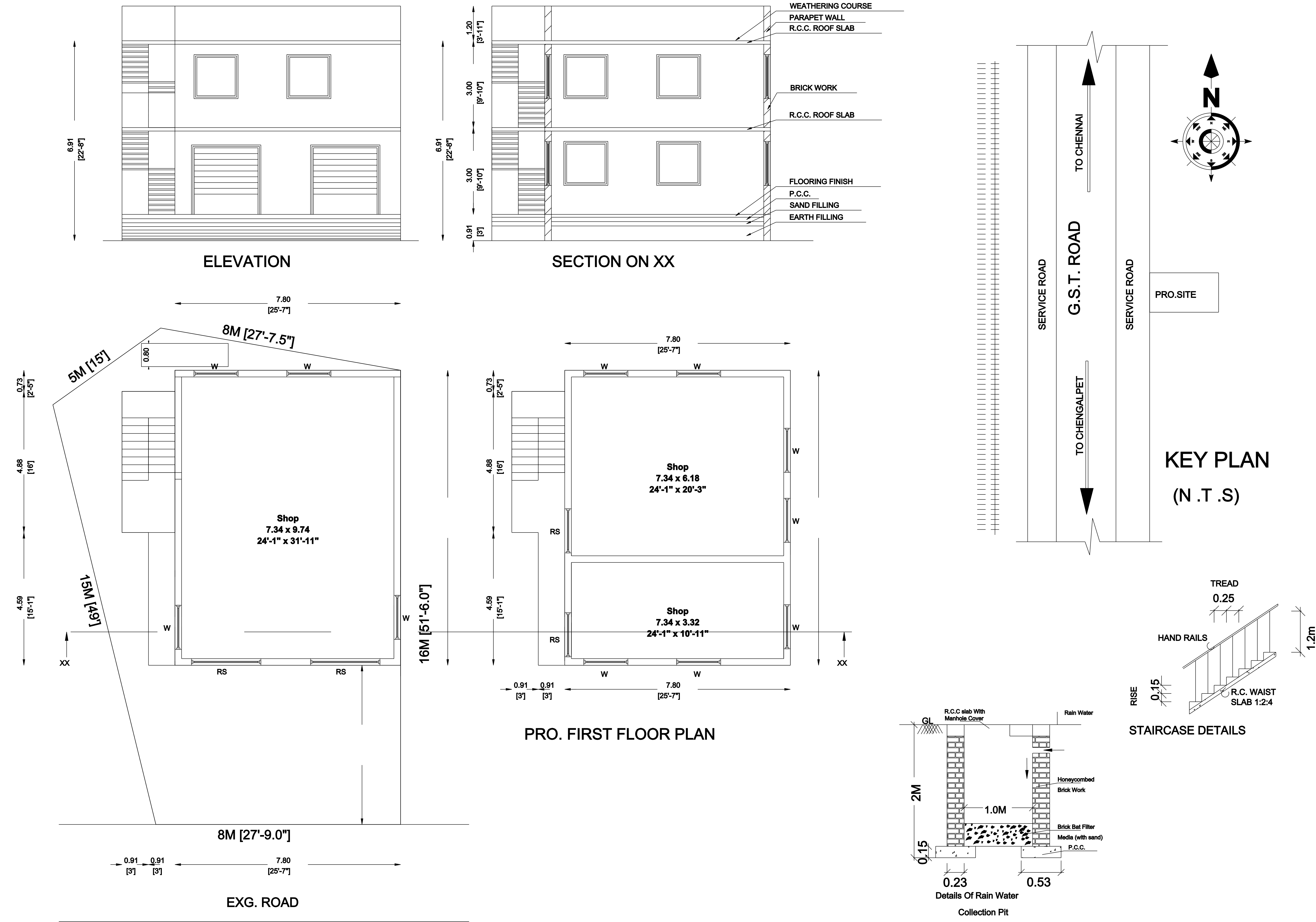
SITE CUM EXG. GROUND FLOOR PLAN
