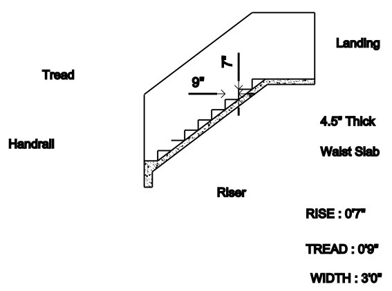
STAIRCASE DETAIL
