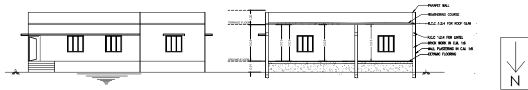
FRONT ELEVATION
