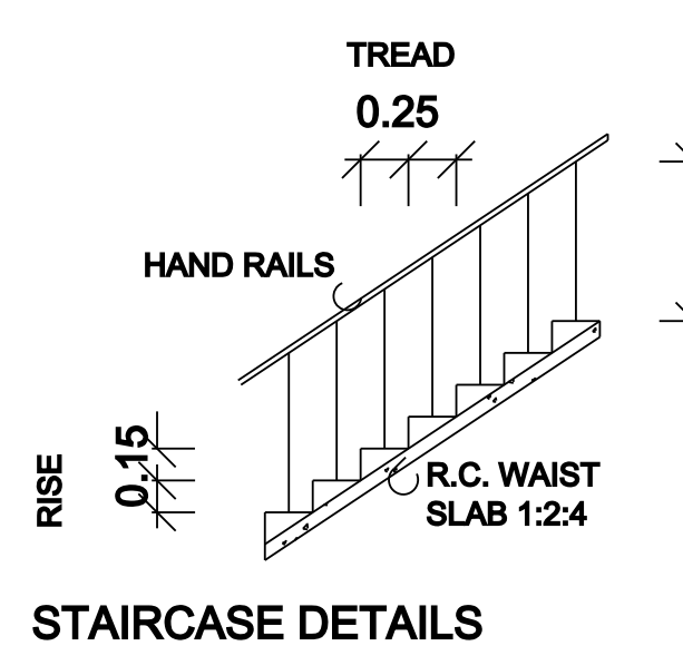
STAIRCASE DETAILS
