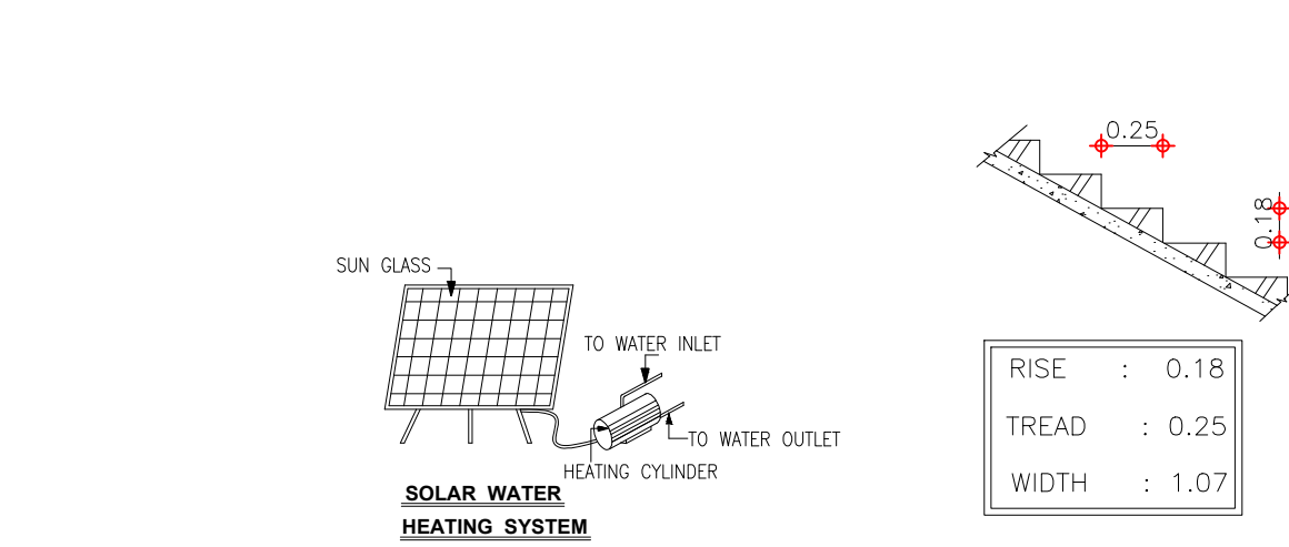
STAIRS DETAILS
