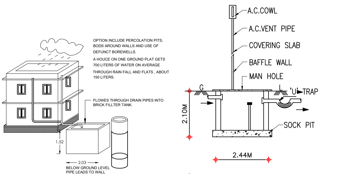
BORE (OR) WELL AND RAIN WATER STORAGE DETAILS
