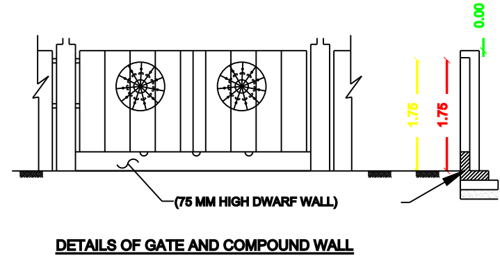
DETAILS OF GATE AND COMPOUND WALL
