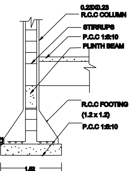
COLUMN DETAILS
