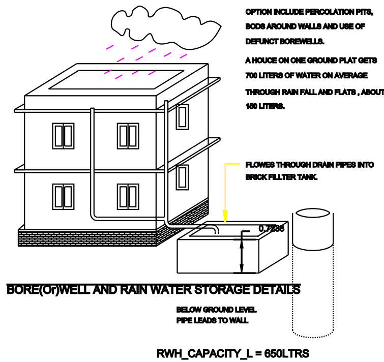
BOREWELL AND RAIN WATER STORAGE DETAILS
