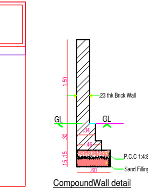
CompoundWall detail
