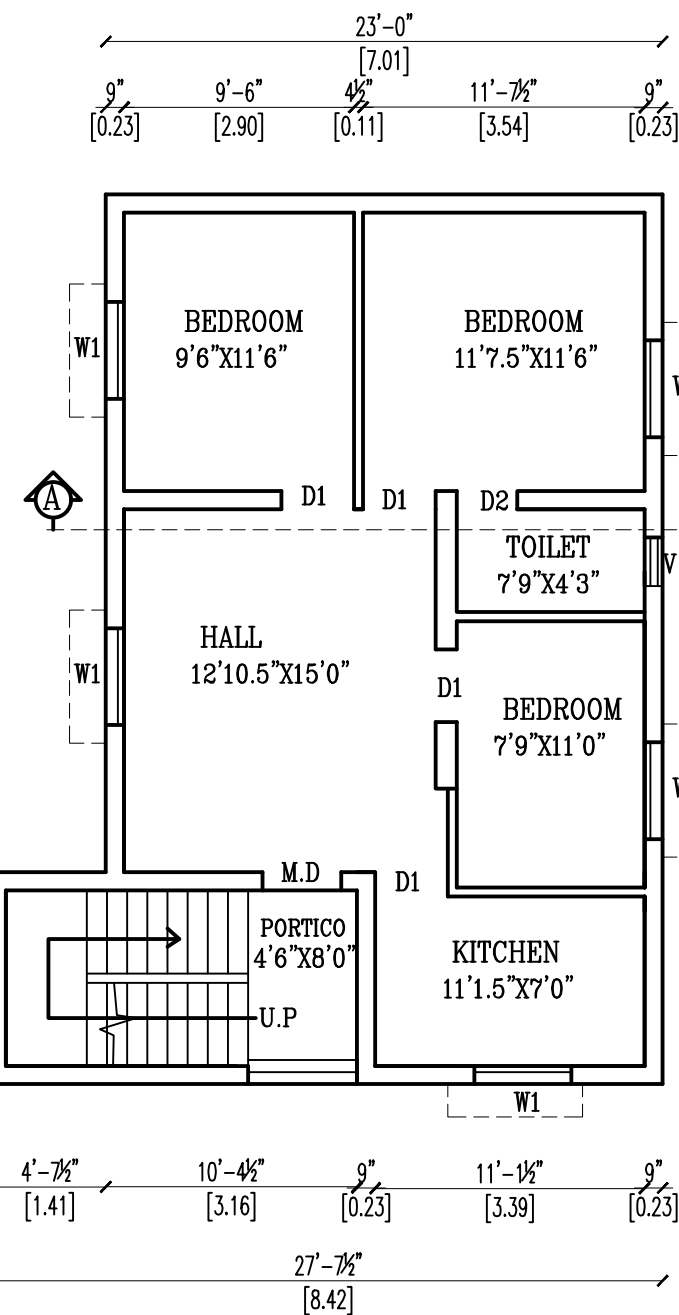
PRO. GROUND FLOOR PLAN
