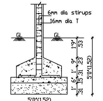
COLUMN FOUNDATION DETAIL SCALE (1:100)
