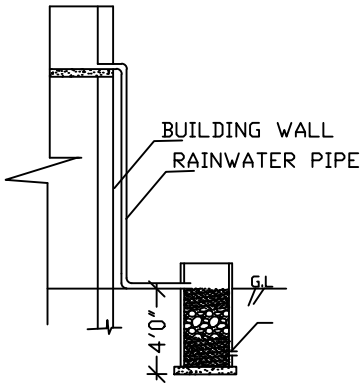
SEC. OF RAIN WATER HARVEST
