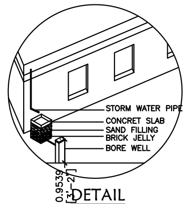
RAINWATER HARVESTING
