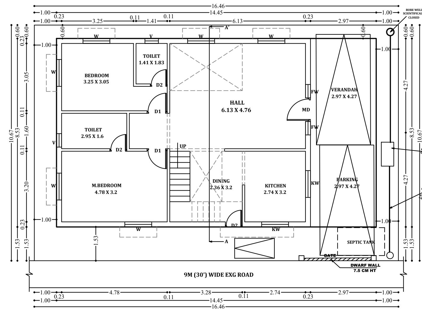
SITE CUM GROUND FLOOR PLAN
