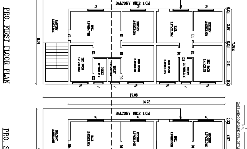
PRO. SITE / GROUND FLOOR PLAN
