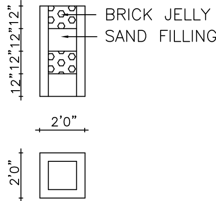
PERCULATION PIT
