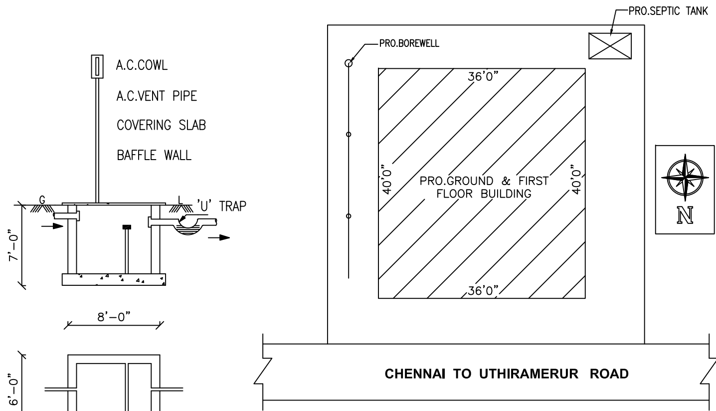
SITE PLAN
