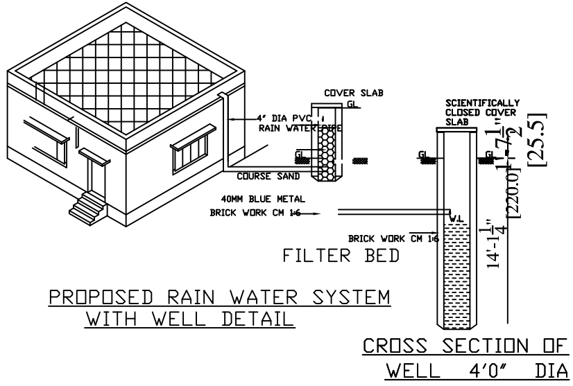
SECTION 1-1
