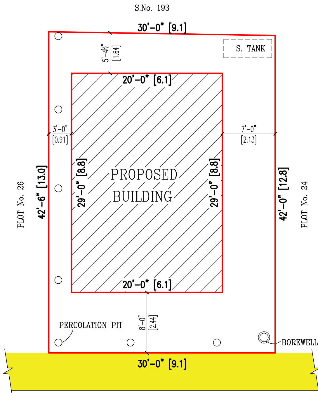
SITE PLAN
