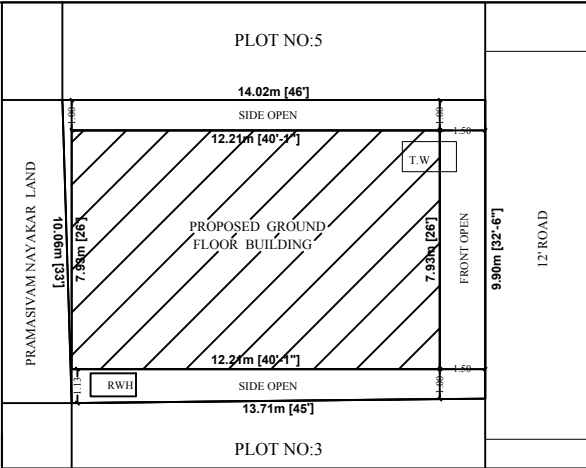
SITE PLAN
