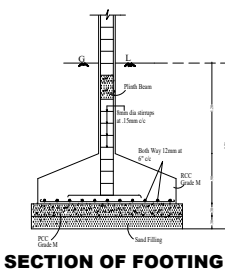
SECTION OF FOOTING
