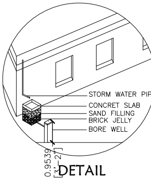
RAINWATER HARVESTING
