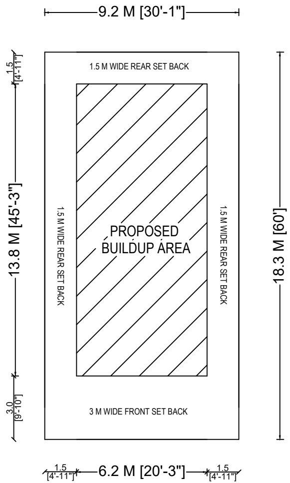
SITE CUM PROPOSED BUILDUP AREA
