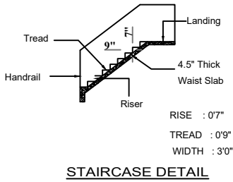
STAIRCASE DETAIL
