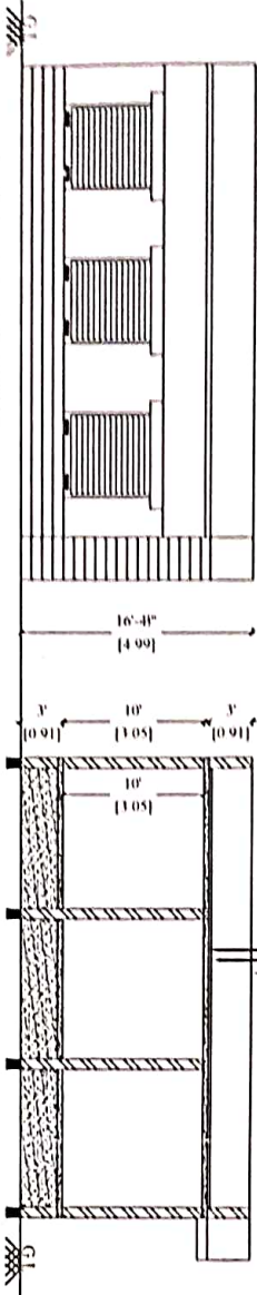
FRONT ELEVATION
