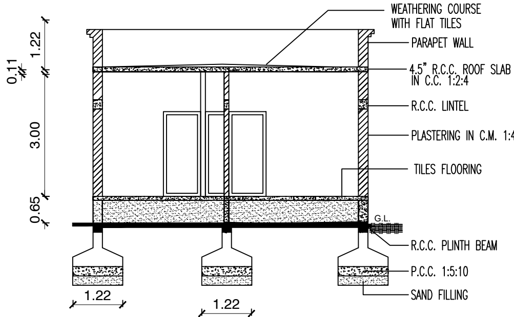
SECTION ON 'A-A' (PROPOSED)
