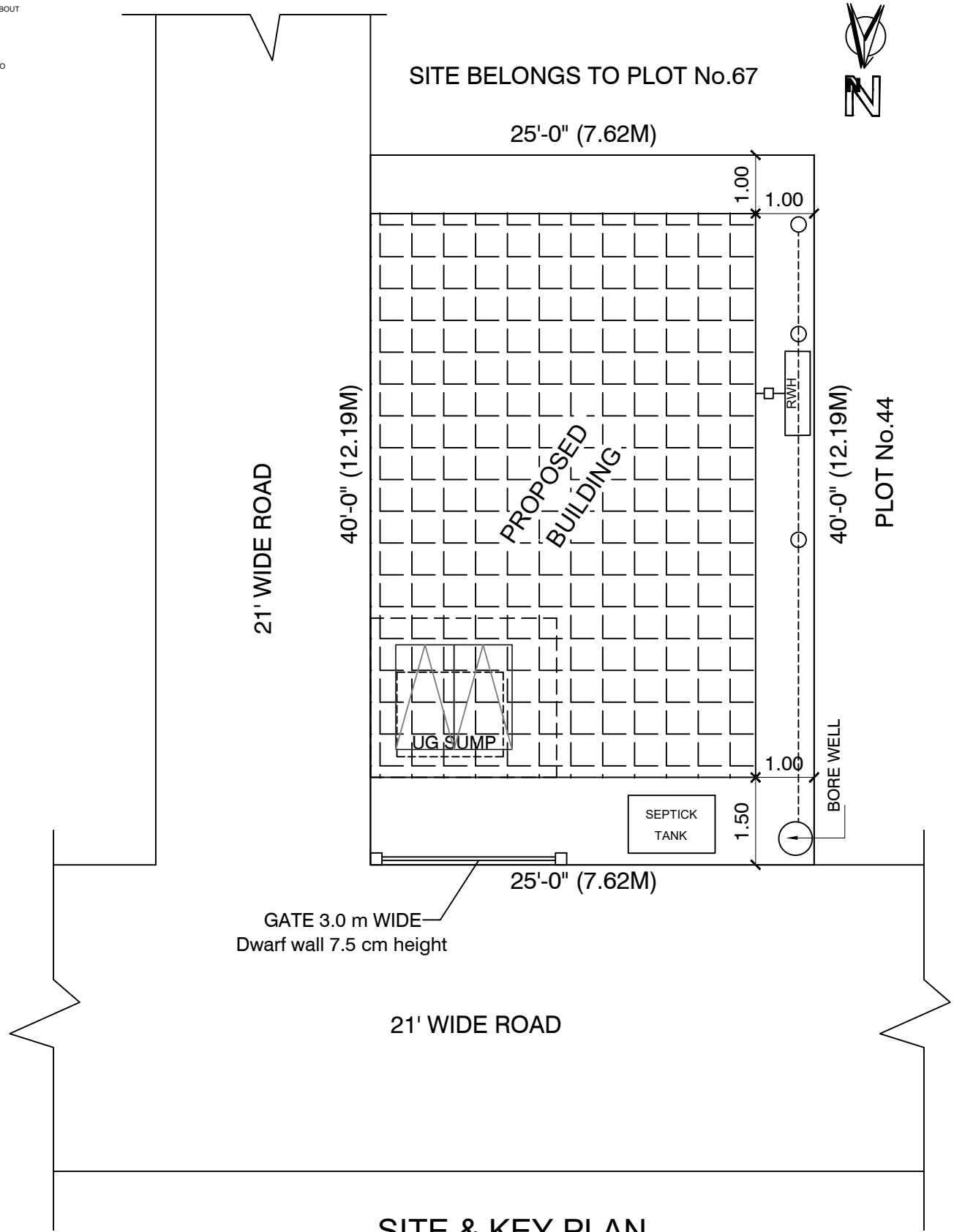
SITE & KEY PLAN SCALE:1:100
