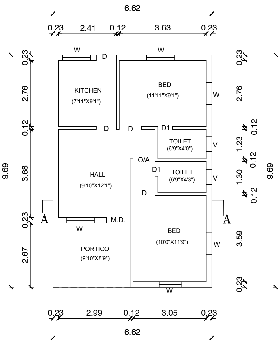
GROUND FLOOR PLAN (PROPOSED)
