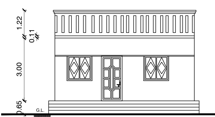
ELEVATION (PROPOSED)
