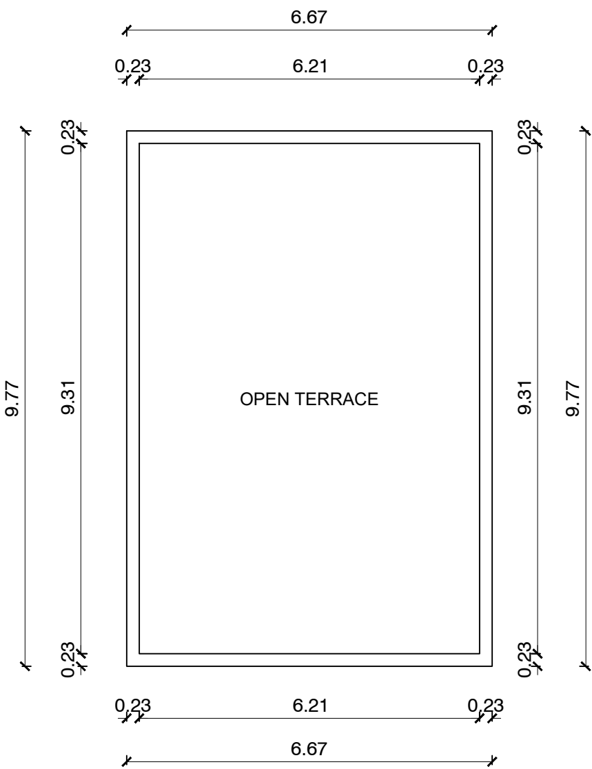
TERRACE FLOOR PLAN (PROPOSED)
