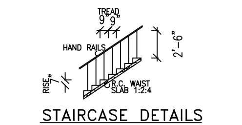
STAIRCASE DETAILS
