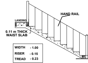
STAIRCASE DETAIL
