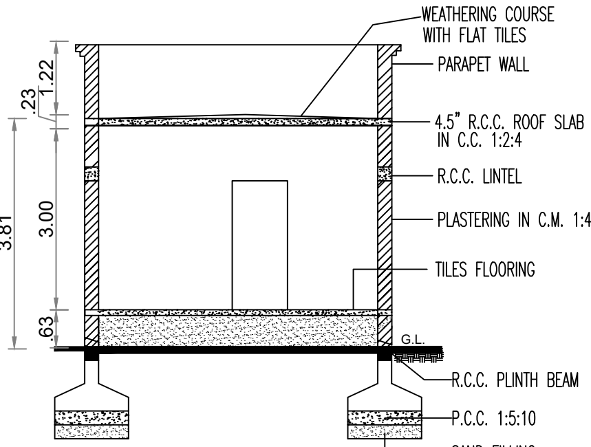
SECTION ON 'A-A' (PROPOSED)
