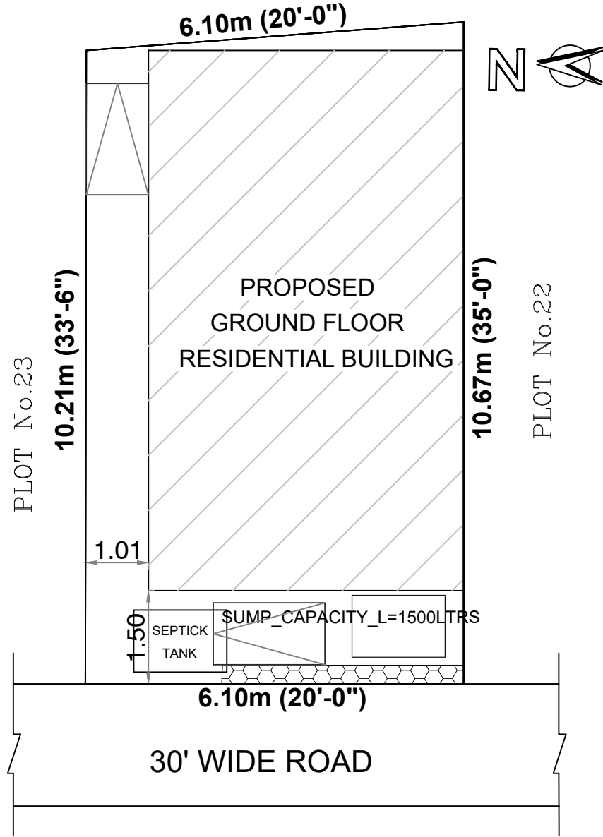
SITE PLAN (1:100)
