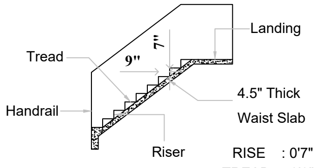
STAIRCASE DETAIL
