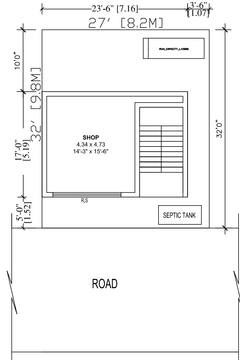
SITE CUM GROUND FLOOR PLAN
