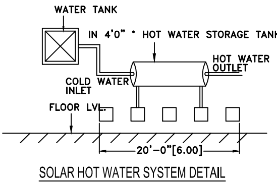
SOLAR HOT WATER SYSTEM DETAIL
