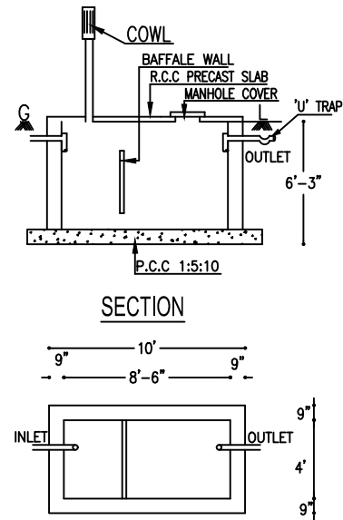
PLAN DETAILS OF SEPTIC TANK
