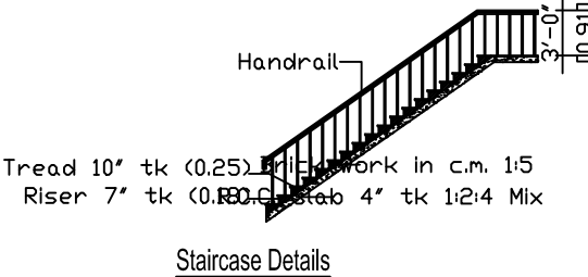
Staircase Details
