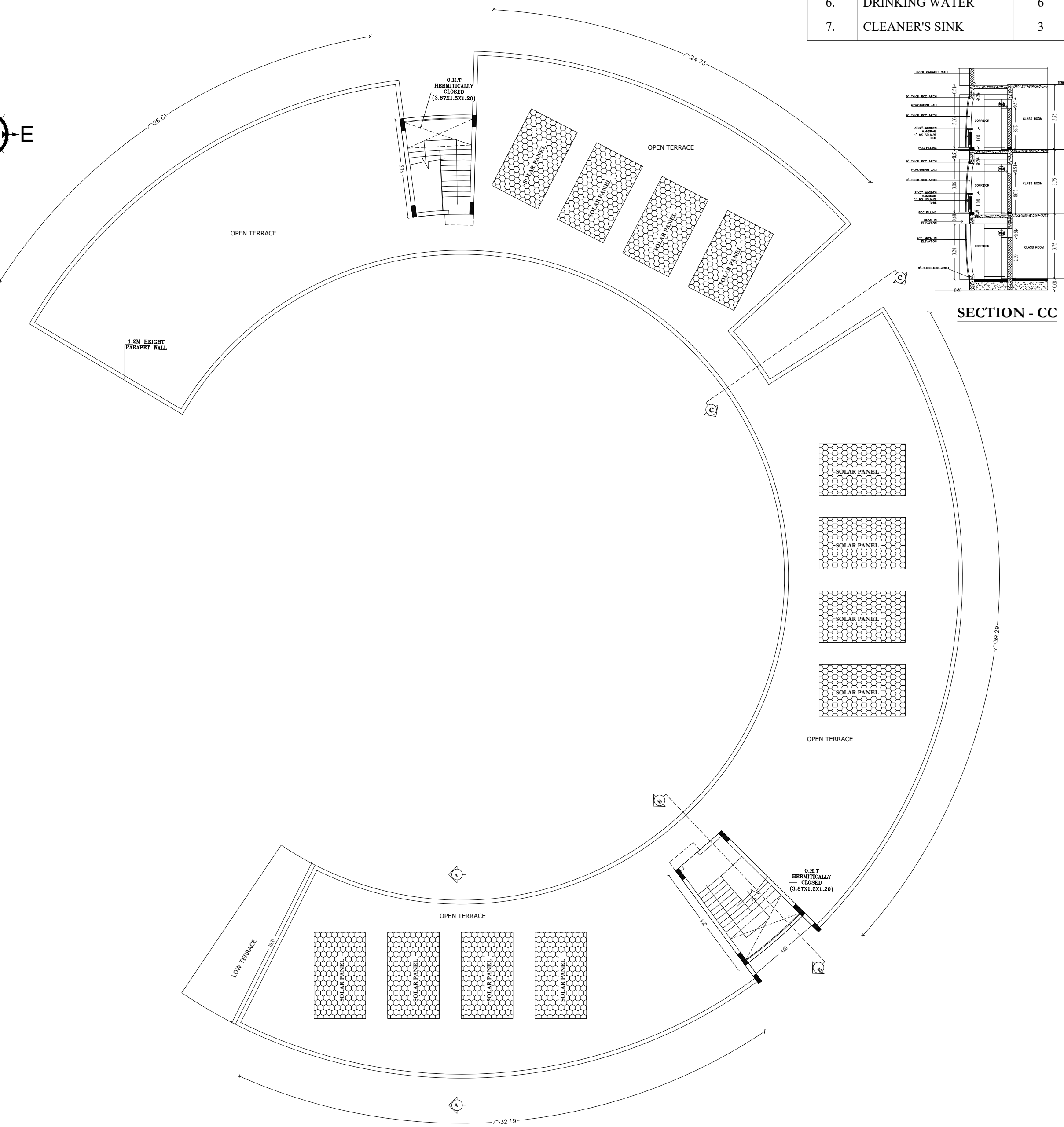
PROPOSED TERRACE FLOOR PLAN
