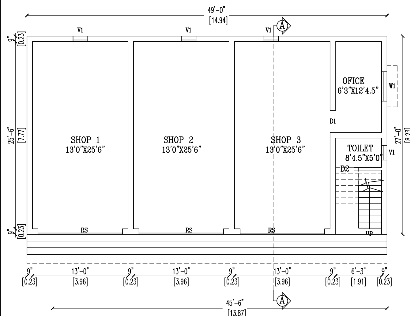
PRO. GROUND FLOOR PLAN
