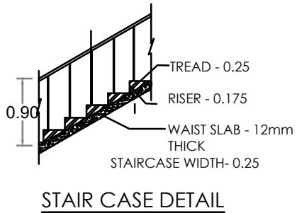
STAIR CASE DETAIL
