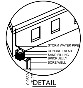
DETAIL RAINWATER HARVESTING
