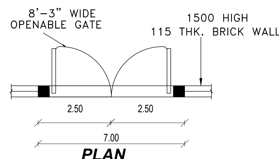
COMPOUND WALL DETAIL
