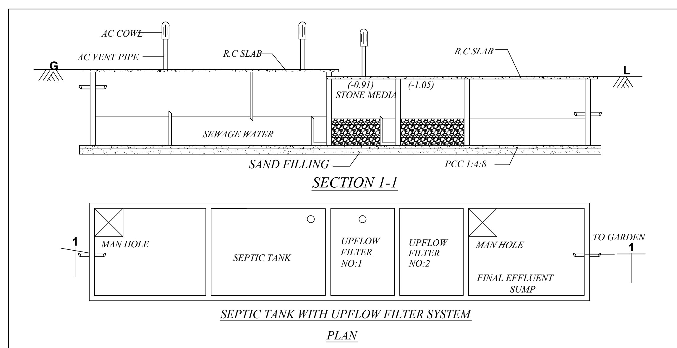
PLAN
