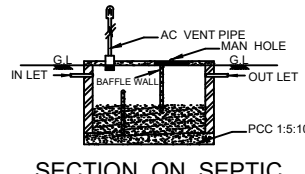
SECTION ON SEPTIC TANK
