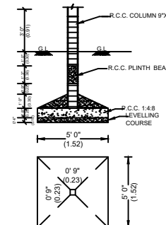
FOUNDATION DETAILS (SCALE 1: 200)
