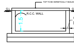
RWHT_CAPACITY_L= 5000LTRS
