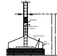
SECTION OF FOOTING
