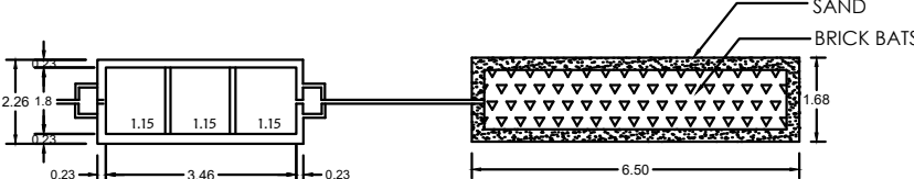
SEPTIC TANK AND TRENCH
