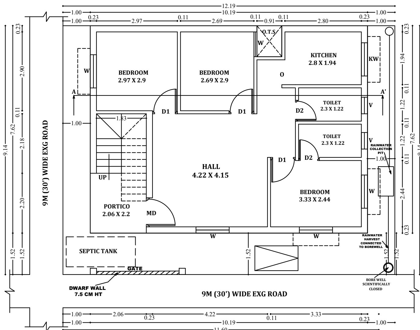
SITE CUM GROUND FLOOR PLAN
