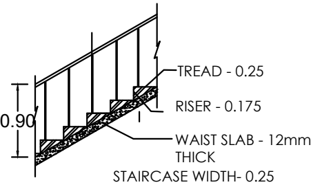
STAIR CASE DETAIL
