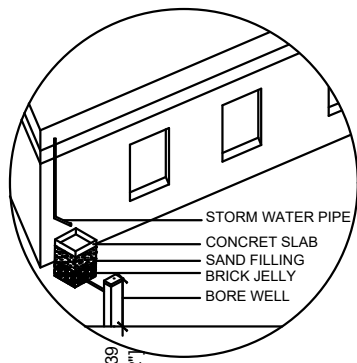
RAINWATER HARVESTING
