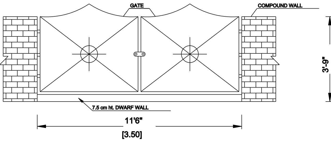
GATE AND COMPOUND WALL DETAILS
