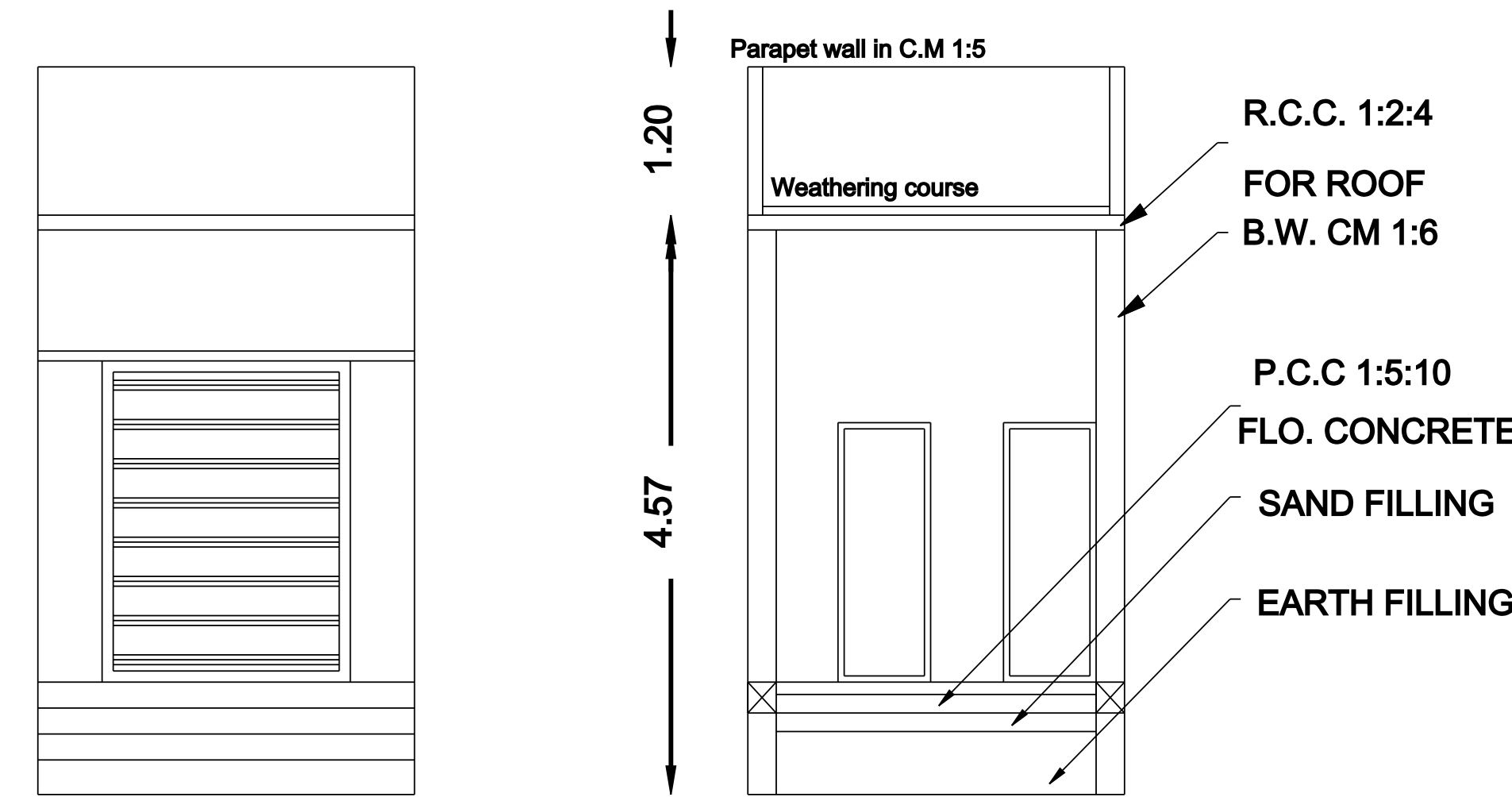
ELEVATION SECTION ON XX
