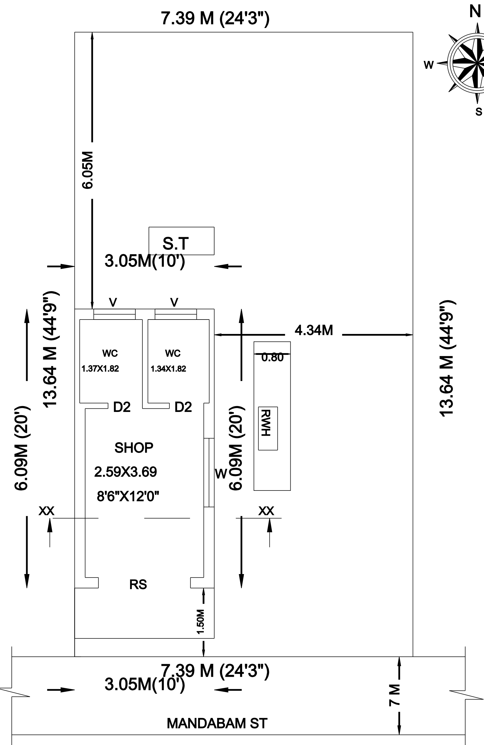
SITE CUM PRO. GROUND FLOOR PLAN
