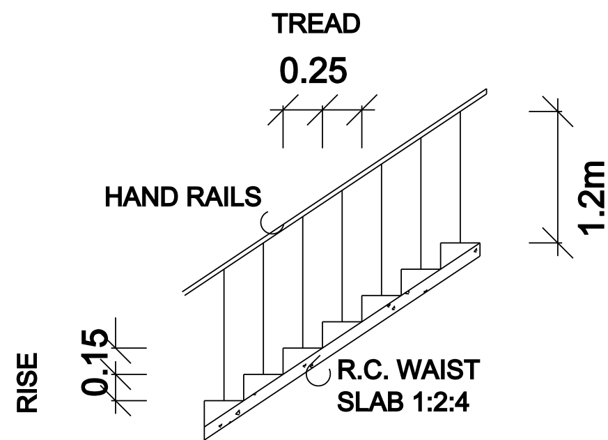
STAIRCASE DETAILS
