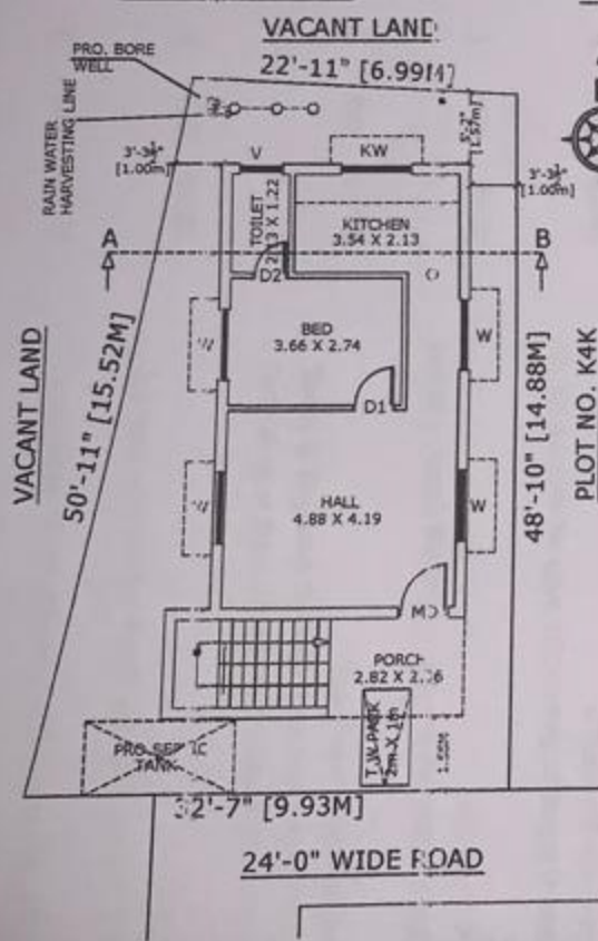
SITE CUM PRO. GROUND FLOOR PLAN
