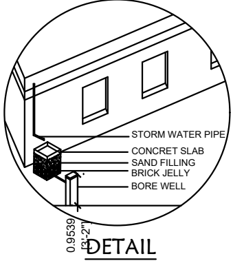
RAINWATER HARVESTING
