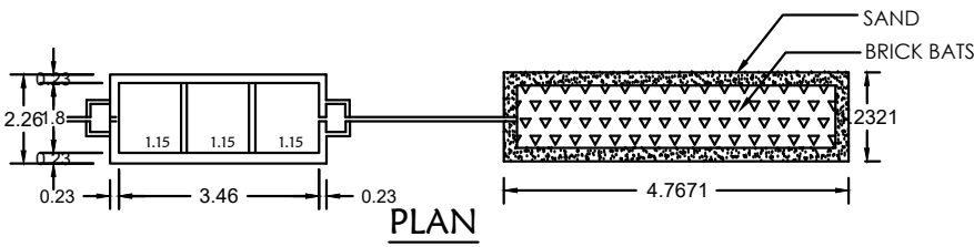
PLAN SEPTIC TANK AND TRENCH
