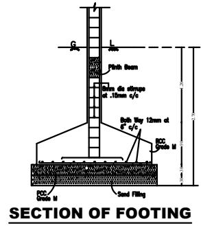
SECTION OF FOOTING
