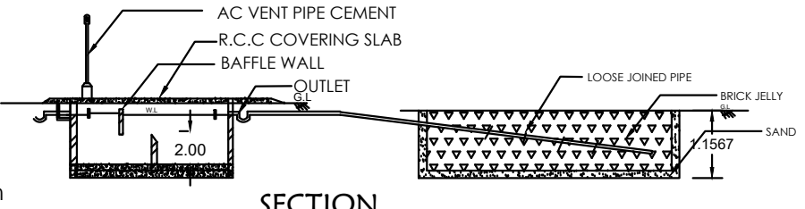
SECTION
