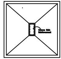
COLUMN FOUNDATION DETAIL PLAN OF FOOTING
