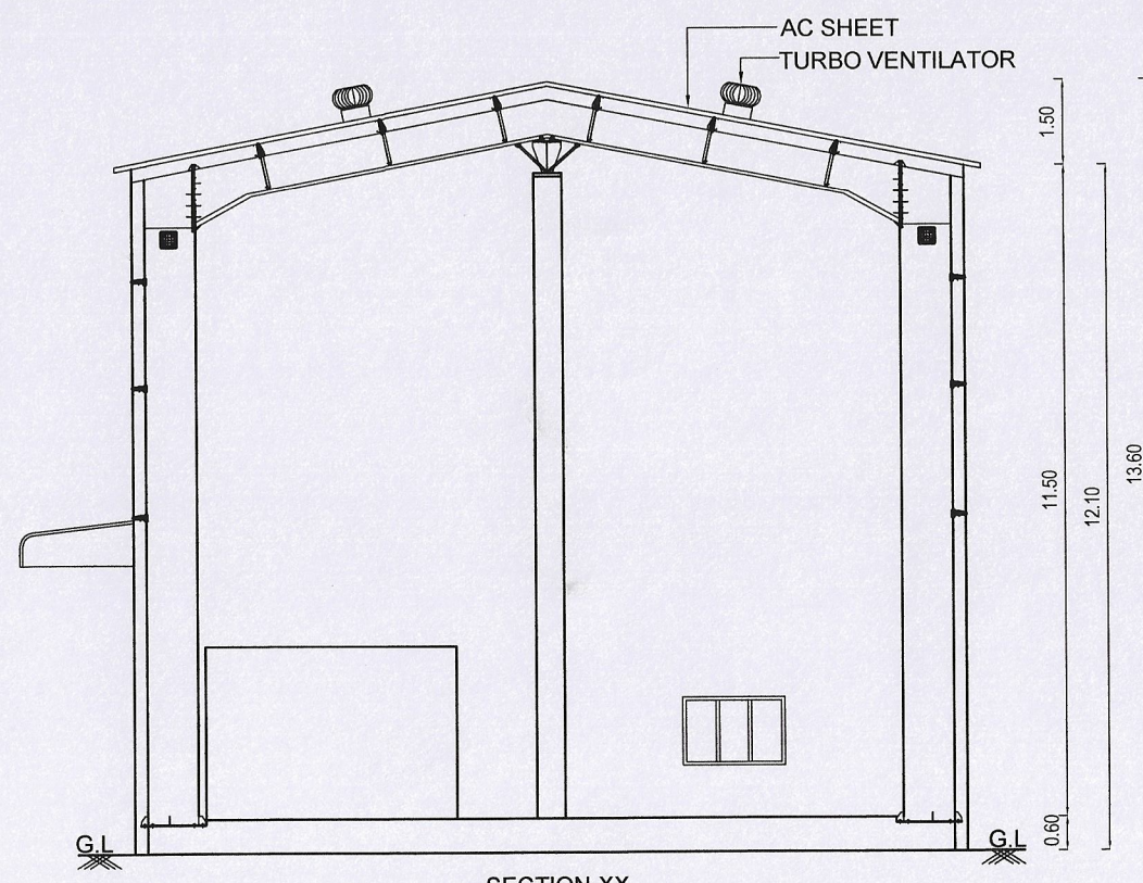
SECTION-XX
