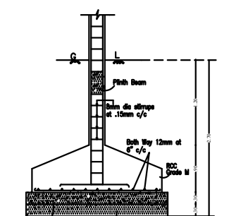
SECTION OF FOOTING
