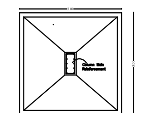
COLUMN FOUNDATION DETAIL
