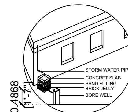
DETAIL RAINWATER HARVESTING
