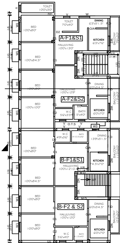
EXG. FIRST FLOOR PLAN
