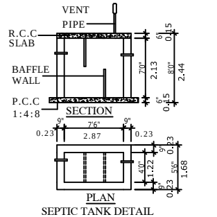
SEPTIC TANK DETAIL
