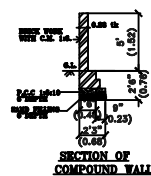
SECTION OF COMPOUND WALL
