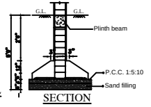
SECTION
