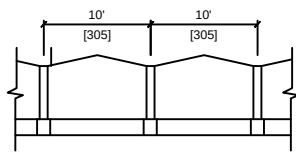
COMPOUND WALL DETAILS
