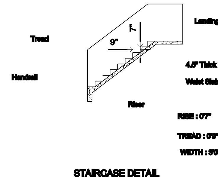
STAIRCASE DETAIL
