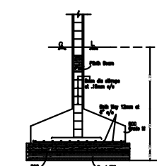
SECTION OF FOOTING
