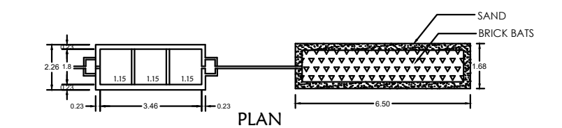
SEPTIC TANK AND TRENCH
