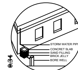
DETAIL RAINWATER HARVESTING
