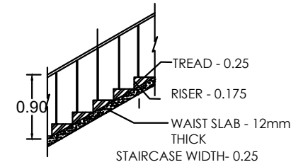
STAIR CASE DETAIL
