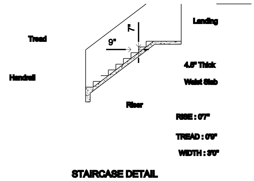
STAIRCASE DETAIL
