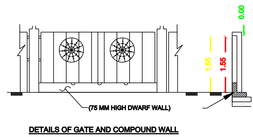
DETAILS OF GATE AND COMPOUND WALL
