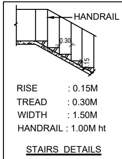
STAIRS DETAILS
