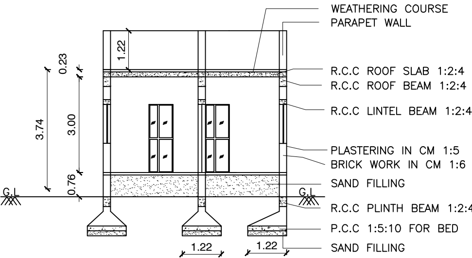
SECTION ON 'A-A' (PROPOSED)
