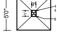
DETAIL OF COLUMN C1,C2
