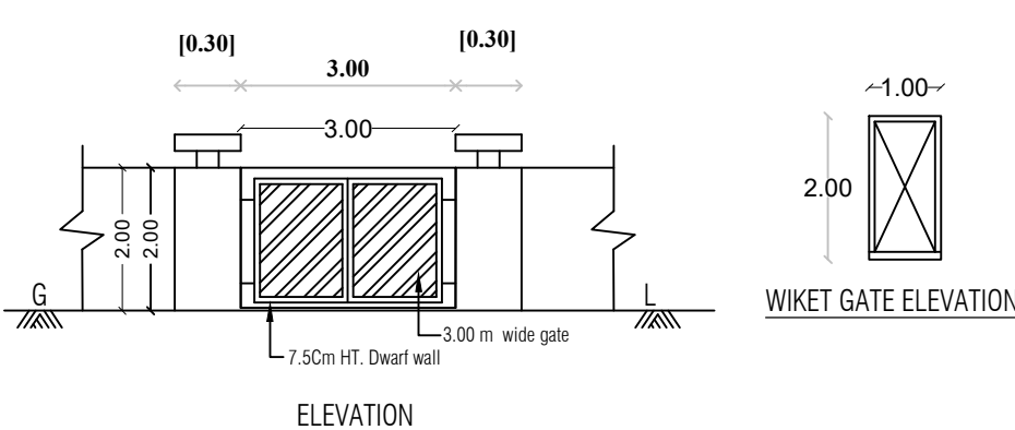
ELEVATION COMPOUND WALL & GATE DETAILS
