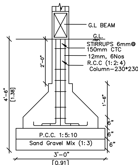
R.C.C. COLUMN FOOTING DETAILS SCALE : 1:25
