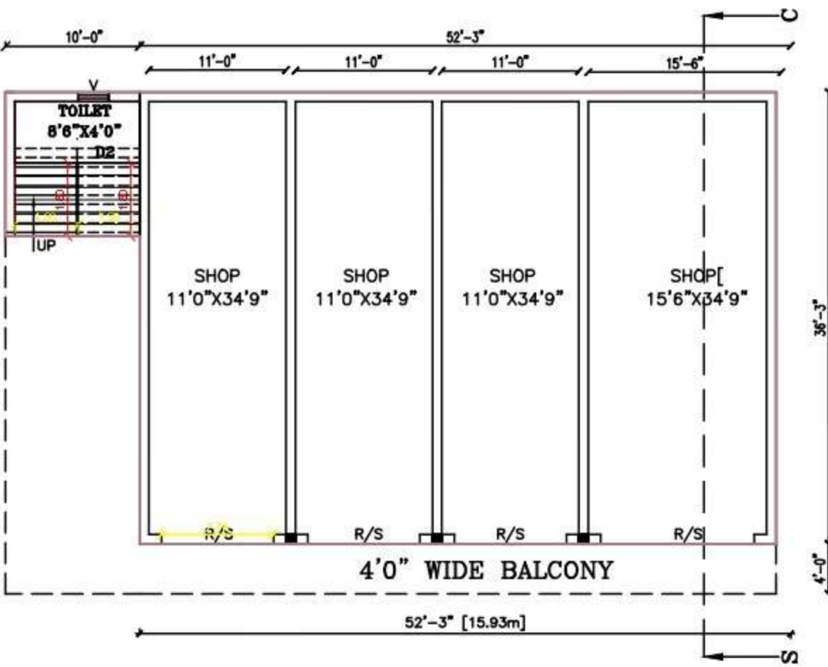
EXTG. GROUND FLOOR PLAN
