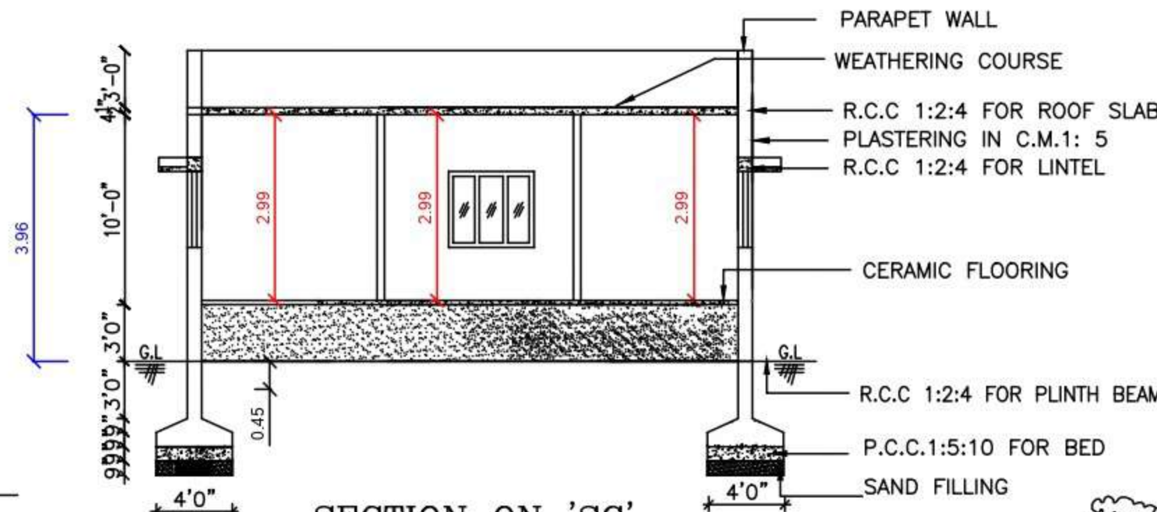
SECTION ON 'SC'
