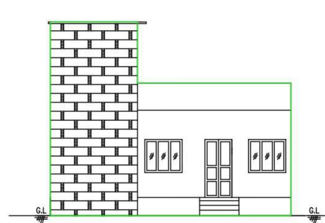
FRONT ELEVATION
