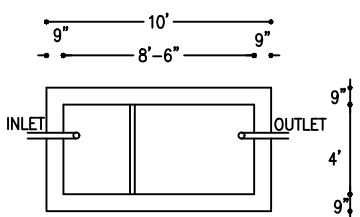
PLAN DETAILS OF SEPTIC TANK
