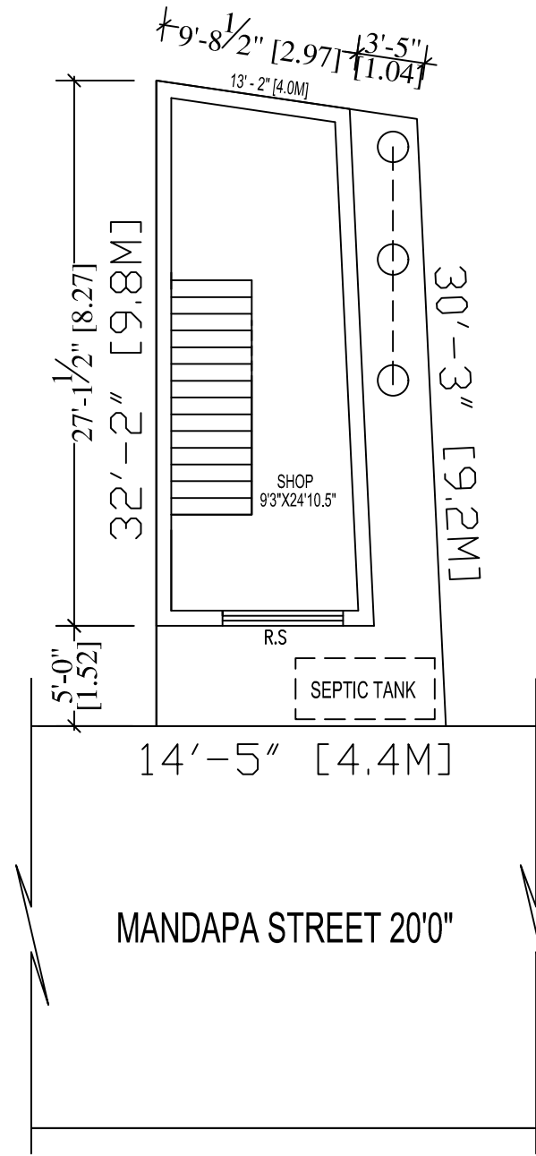
SITE CUM GROUND FLOOR PLAN
