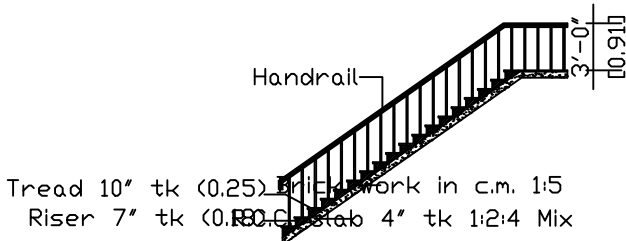
Staircase Details
