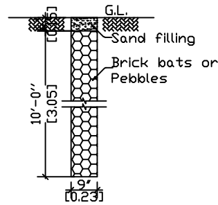
Percolation Pit
