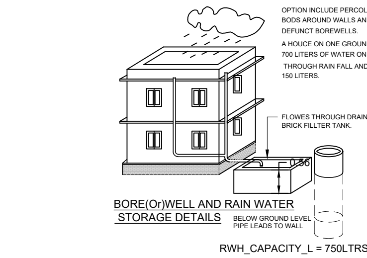
BORE(O)WELL AND RAIN WATER STORAGE DETAILS
