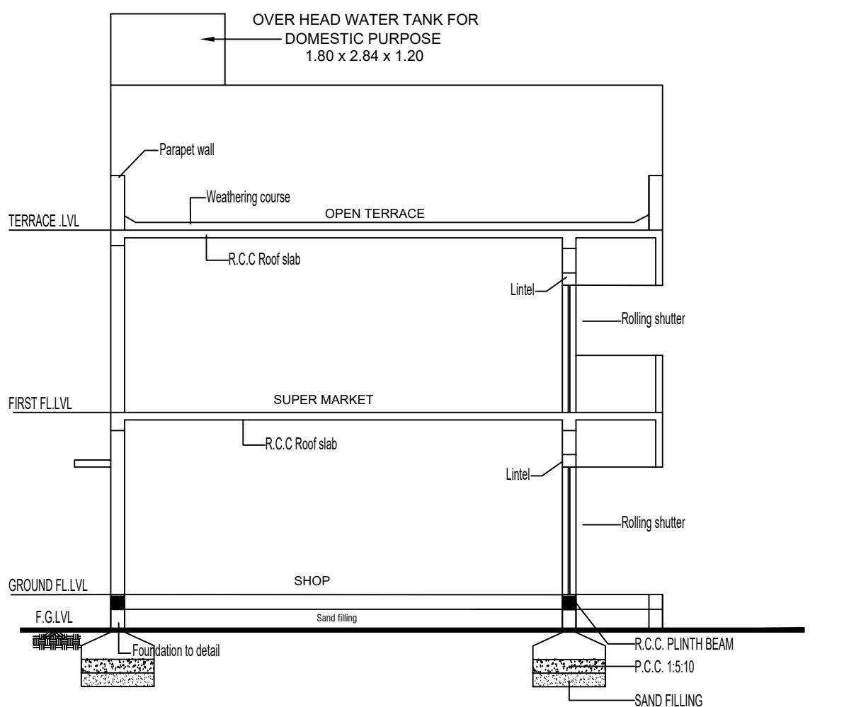
SECTION - AA' (PROPOSED)
