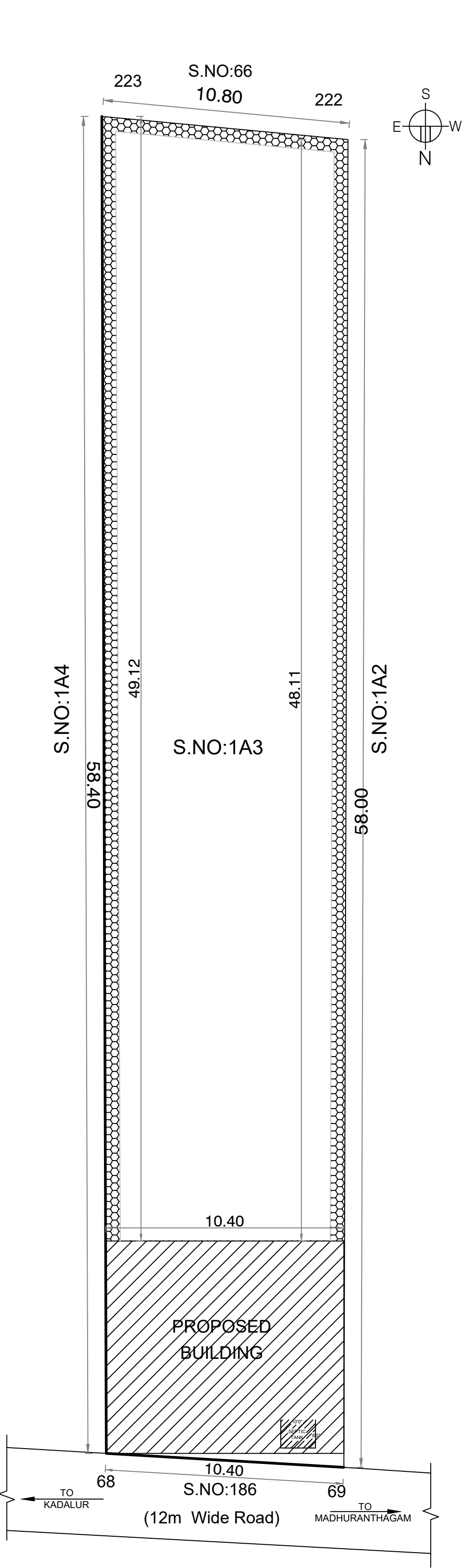
SITE PLAN (SCALE : 1" = 16'0")
