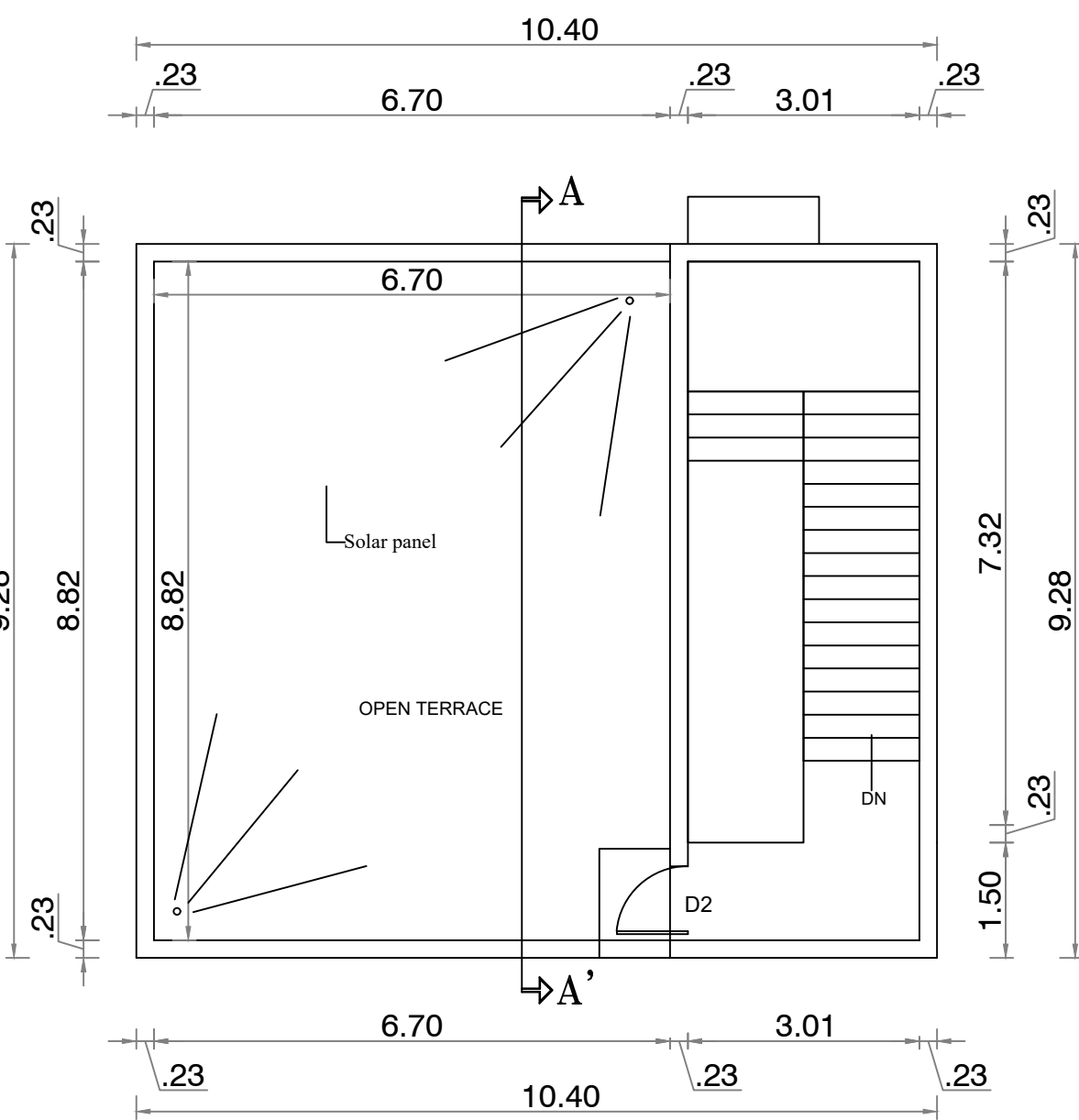
TERRACE FLOOR PLAN (PROPOSED)
