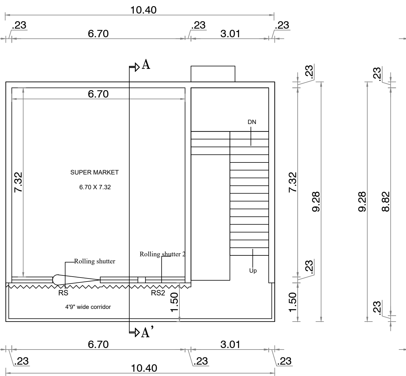
FIRST FLOOR PLAN (PROPOSED)
