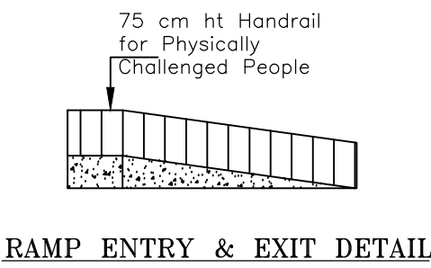
RAMP ENTRY & EXIT DETAIL
