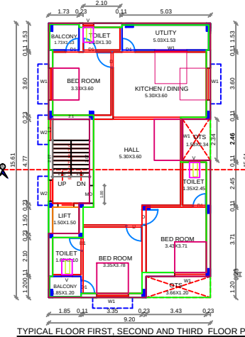
TYPICAL FLOOR FIRST, SECOND AND THIRD FLOOR PLAN
