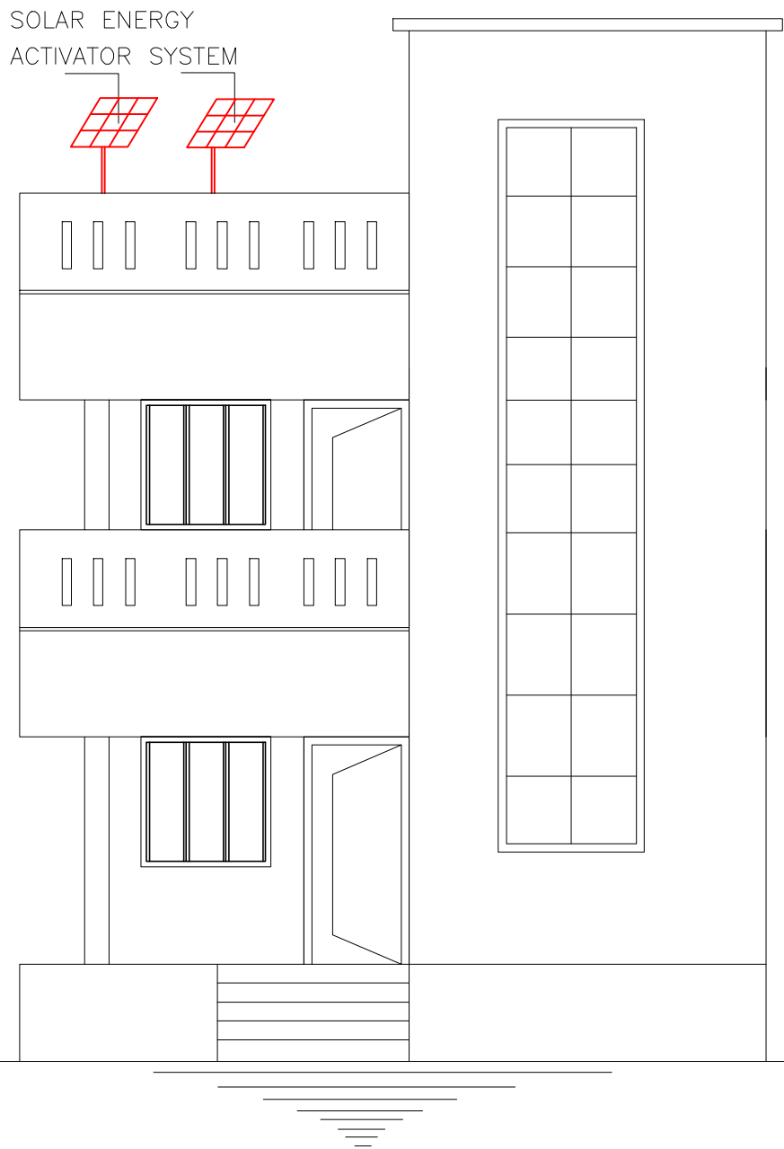
FRONT ELEVATION
