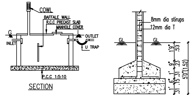
DETAILS OF SEPTIC TANK
