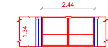
ELEVATION OF COMPOUND WALL
