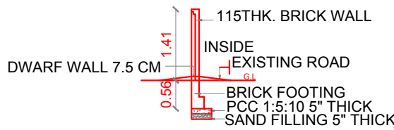
SECTION OF COMPOUND WALL
